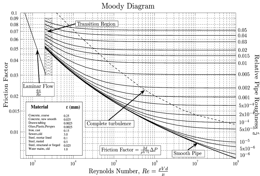
Gambar 2. Diagram Moody
