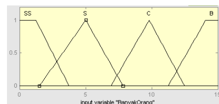
Gambar 4 Input Membership Function BanyakOrang
