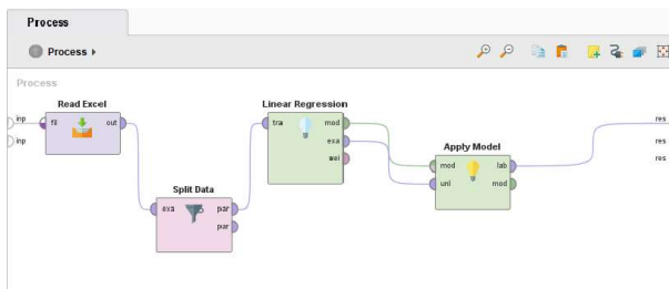
Gambar 5. Proses Rapidminer
