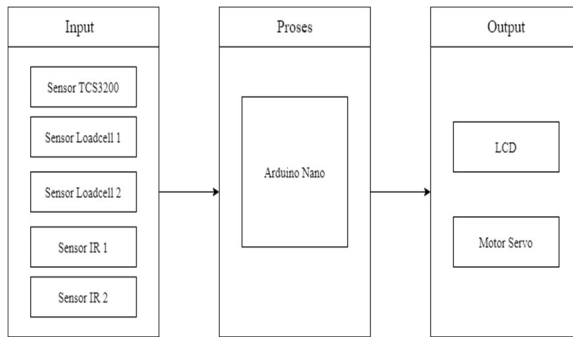
Gambar 2. Blok Diagram
