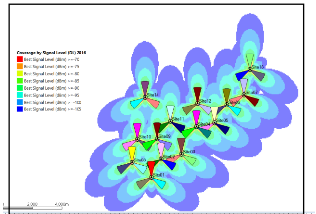
Gambar 8. Coverage By Signal Level
