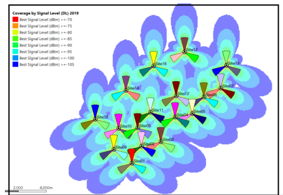
Gambar 20. Coverage By Signal Level
