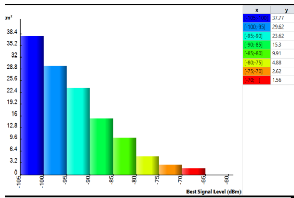
Gambar 21. Histogram by covered areas
