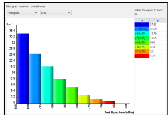
Gambar 13. Histogram by covered areas
