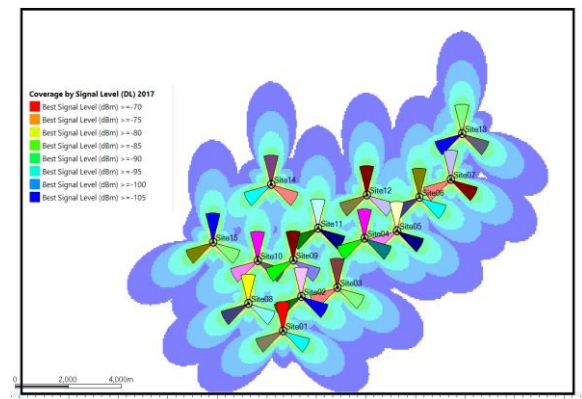
Gambar 12. Coverage By Signal Level
