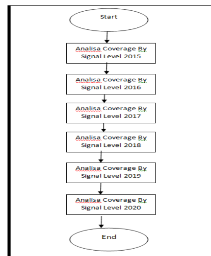
Gambar 3. Flowchart Penelitian
