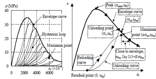
Gambar 3: Hysteresis Loop
