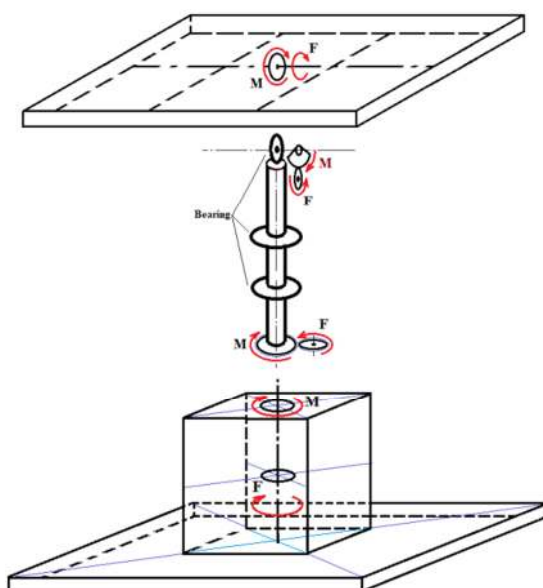
Gambar 5. Desain awal solar tracker dual axis .
