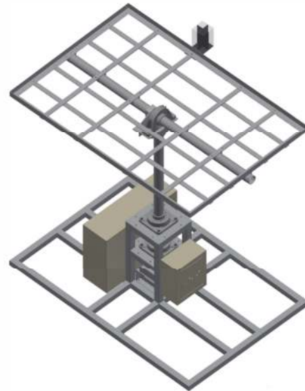
Gambar 10. Desain solar tracker dual axis .
