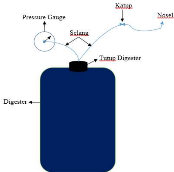
Gambar 1. Instalasi peralatan penelitian
