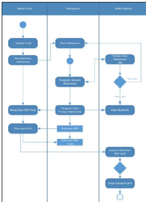
Gambar 4. Activity Diagram SKPI
