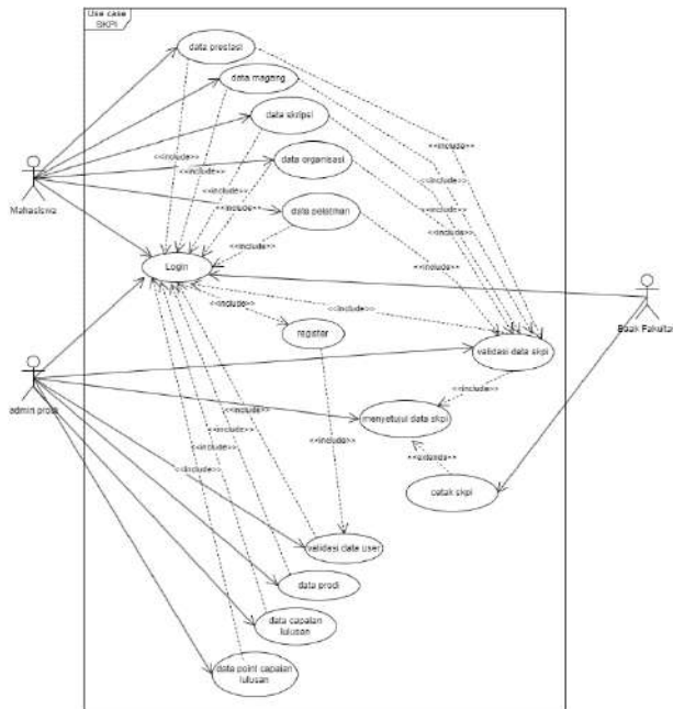
Gambar 3. Use Case Diagram SKPI
