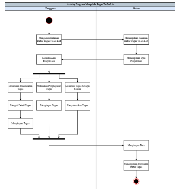
Gambar 5. Activity Diagram Mengelola Tugas
