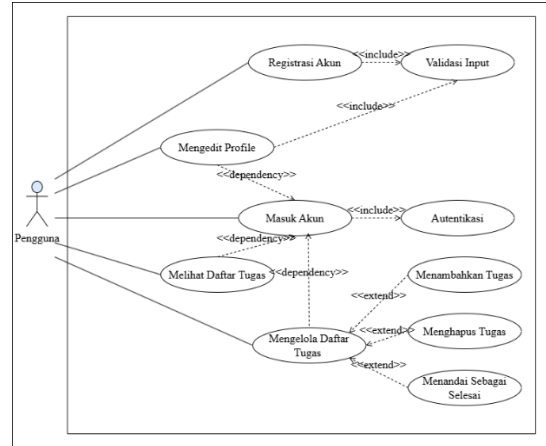
Gambar 2. Use Case Diagram Sistem To-Do List
