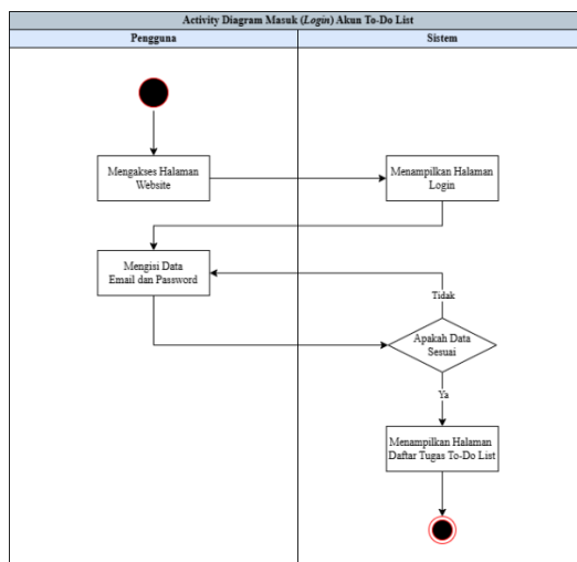
Gambar 4. Activity Diagram Masuk Akun
