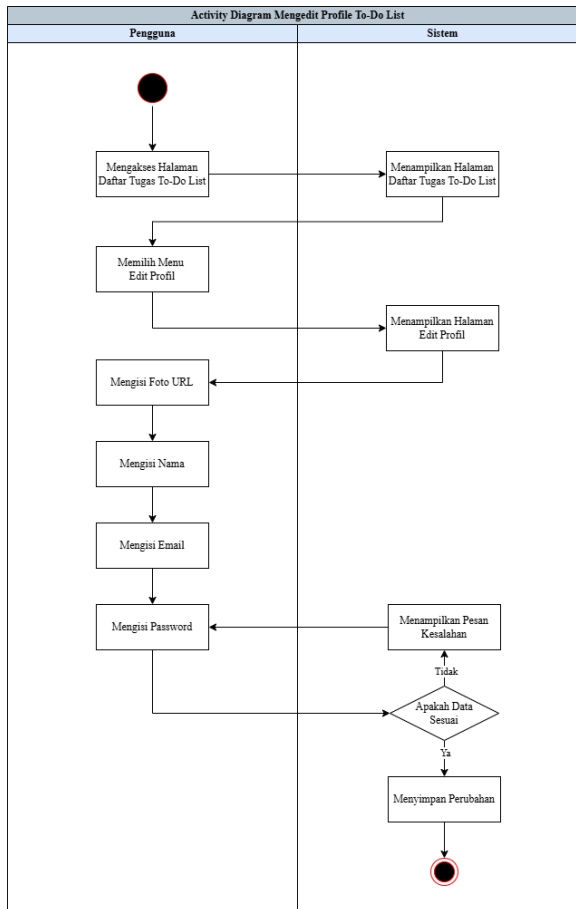
Gambar 6. Activity Diagram Mengedit Profil
