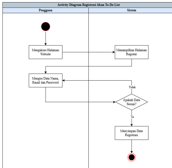
Gambar 3. Activity Diagram Registrasi Akun
