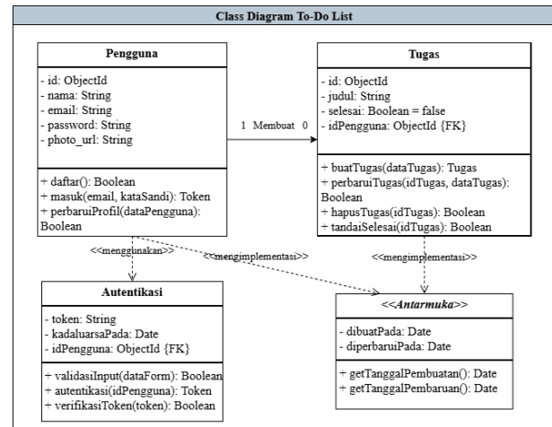
Gambar 7. Class Diagram Sistem To-Do List
