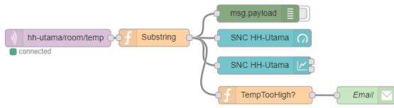
Gambar 13. Sistem Monitoring SNC HH-Utama
