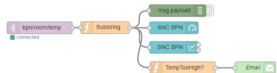
Gambar 12. Sistem Monitoring SNC BPN
