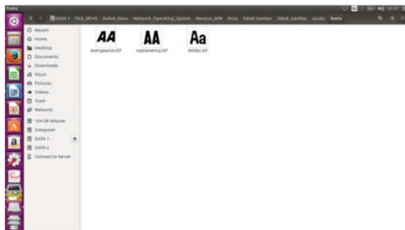
Gambar 11. File drawable-xhdpi-v4
