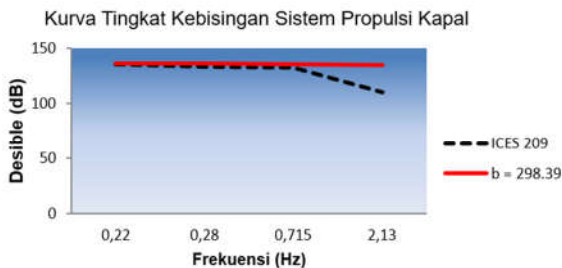
Gambar 5. Kurva kebisingan b = 298,39 mm
