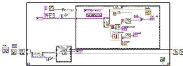
Gambar 4. Block diagram BMS berbasis LabVIEW
