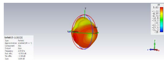
Gambar 15. Gain Antena 3
