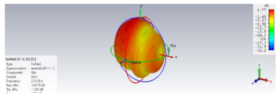
Gambar 6. Gain antena 1
