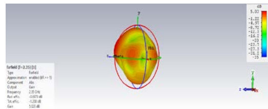
Gambar 13. Gain Antena 1
