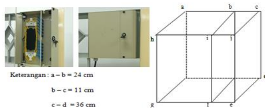
Gambar 3. Optical Terminal Box
