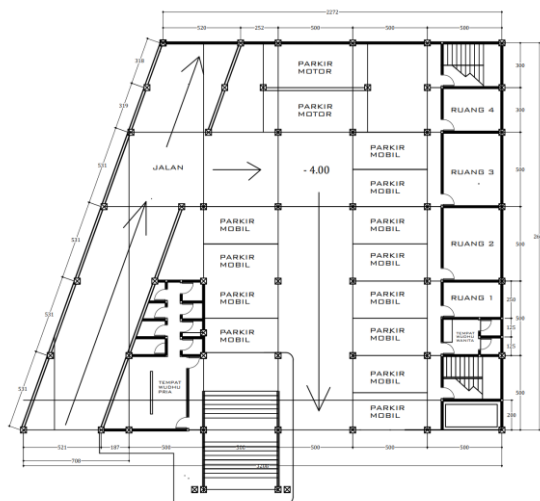
Gambar 4. Denah Basement Masjid Jami' Addin
