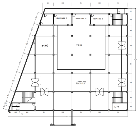
Gambar 6. Denah Lantai 2 Masjid Jami' Addin
