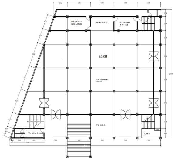
Gambar 5. Denah Lantai 1 Masjid Jami' Addin
