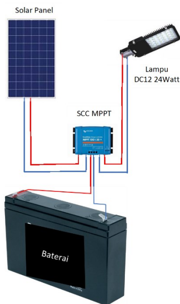
Gambar 3. Wiring diagram panel surya
