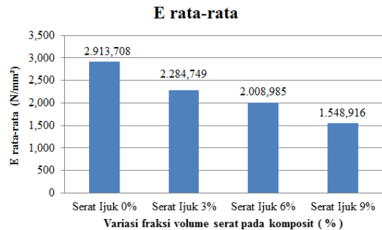
Gambar 9. Diagram modulus elastisitas tarik
