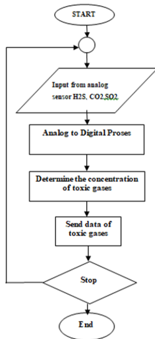
Gambar 3.5 Proses Pendeteksian Gas Beracun
