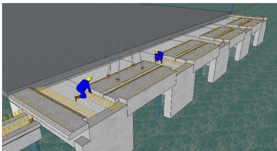
Gambar 16. Ilustrasi Precast Slab Extension Jetty
