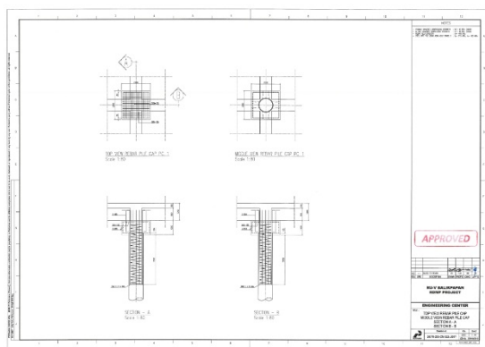
Gambar 5. Top middle view rebar pile cap saat tender
