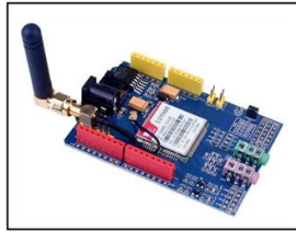
Gambar. 3 Modul SIM900A GSM/GPRS
